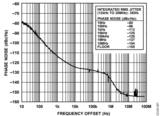
Figure 7. Absolute Phase Noise (Output Driver = 21 mA Mode), f_R = 19.44 MHz, f_{OUT} = 174.703 MHz, DPLL Loop Bandwidth = 1 kHz, f_{SYS} = 49.152 MHz Crystal
