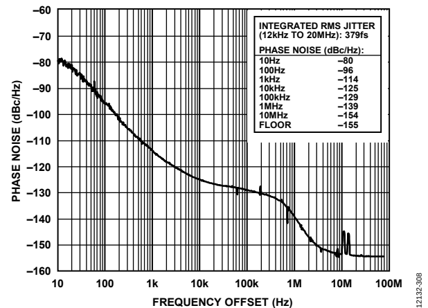
Figure 8. Absolute Phase Noise, f_R = 19.44 MHz, f_{OUT} = 161.1328125 MHz, DPLL Loop Bandwidth = 100 Hz, f_{SYS} = 49.152 MHz Crystal
