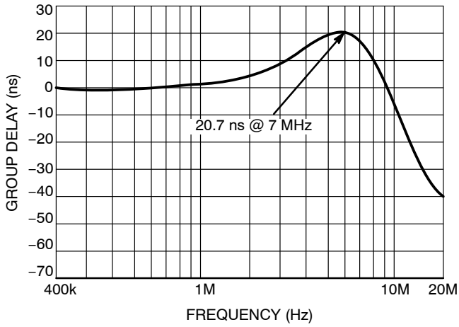
Figure 9. SD Normalized Group Delay
