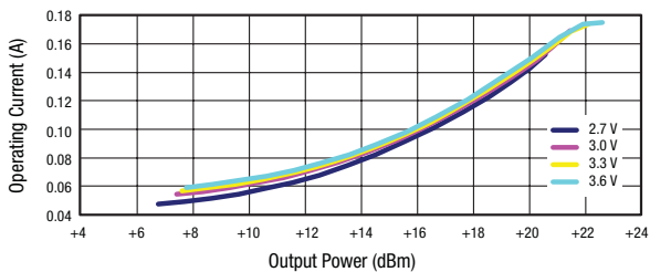
Figure 7. Operating Current vs Output Power Over Voltage @ 2450 MHz (TA = 25 °C)
