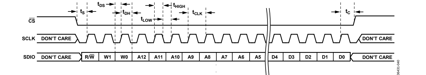
Figure 48. Serial Control Port Write—MSB First, 16-Bit Instruction, Timing Measurements
