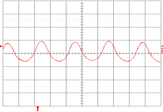
Fig. 13: Input reflected ripple current, i_c (100 mA/div.), measured at input terminals at full rated load current and V_{in} = 48 V. Refer to Fig. 12 for test setup. Time scale: 1 \mu s/div.
