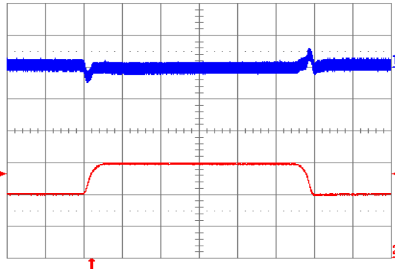
Fig. 9: Output voltage response to load current step-change (10 A – 15 A – 10 A) at V_{in} = 48 V. Top trace: output voltage (100 mV/div.). Bottom trace: load current (5 A/div.). Current slew rate: 0.1 A/ \mu s. C_o = 1 \mu F ceramic. Time scale: 0.2 ms/div.
