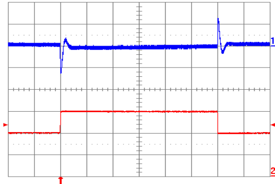
Fig. 10: Output voltage response to load current step-change (10 A – 15 A – 10 A) at V_{in} = 48 V. Top trace: output voltage (100 mV/div.). Bottom trace: load current (5 A/div.). Current slew rate: 5 A/ \mu s. C_o = 470 \mu F POS + 1 \mu F ceramic. Time scale: 0.2 ms/div.
