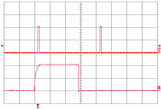
Fig. 16: Load current (top trace, 10 A/div., 50 ms/div.) into a 10 m \Omega short circuit during restart, at V_{in} = 48 V. Bottom trace (10 A/div., 2 ms/div.) is an expansion of the on-time portion of the top trace.
