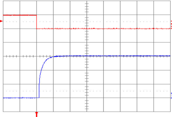
Fig. 7: Turn-on transient at full rated load current (resistive) with no output capacitor at V_{in} = 48 V, triggered via ON/OFF pin. Top trace: ON/OFF signal (5 V/div.). Bottom trace: output voltage (2 V/div.). Time scale: 5 ms/div.
