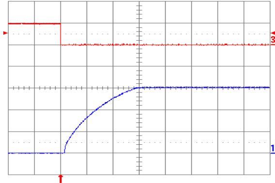
Fig. 8: Turn-on transient at full rated load current (resistive) plus 10,000 \mu F at V_{in} = 48 V, triggered via ON/OFF pin. Top trace: ON/OFF signal (5 V/div.). Bottom trace: output voltage (2 V/div.). Time scale: 5 ms/div.
