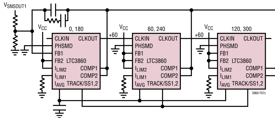
Figure 7c. 6-Phase Operation
