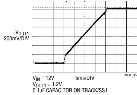
Soft-Start Start-Up
