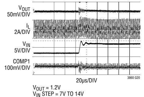
Line Step Transient Response (Single Phase)
