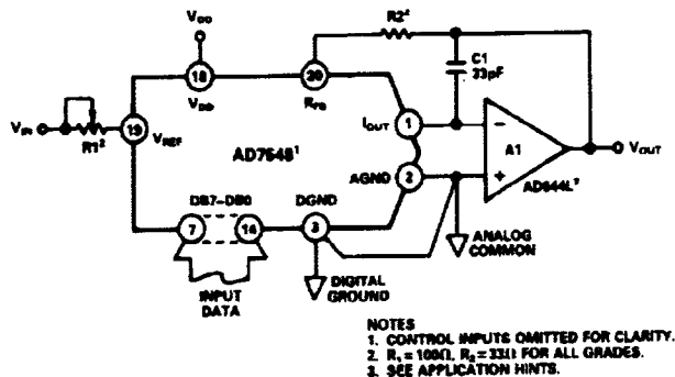
Figure 6. Unipolar Binary Operation
