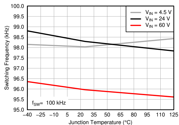
图 5-2. Switching Frequency vs. Junction Temperature ( f_{SW} = 100 \text{ kHz} )
