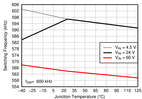
图 5-4. Switching Frequency vs. Junction Temperature ( f_{SW} = 600 \text{ kHz} )
