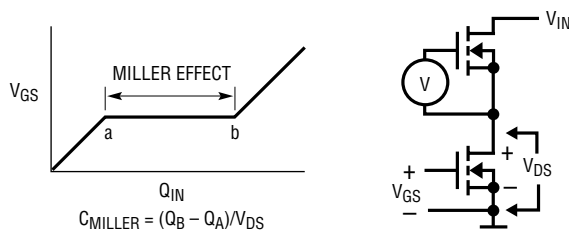
Figure 5. Gate Charge Characteristic
