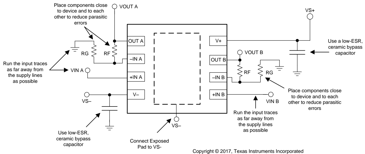
Figure 29. Layout Example
