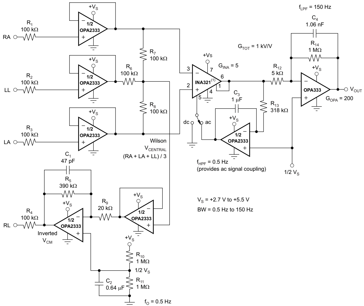
Figure 28. Single-Supply, Very Low Power, ECG Circuit
