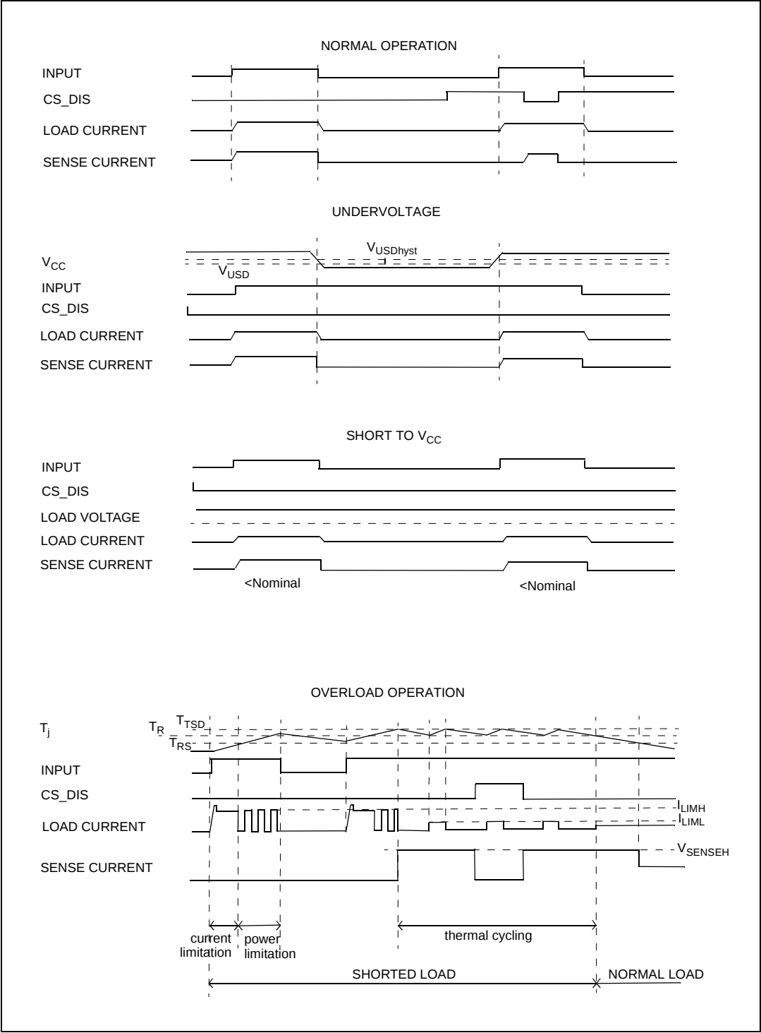
Figure 26. Waveforms
