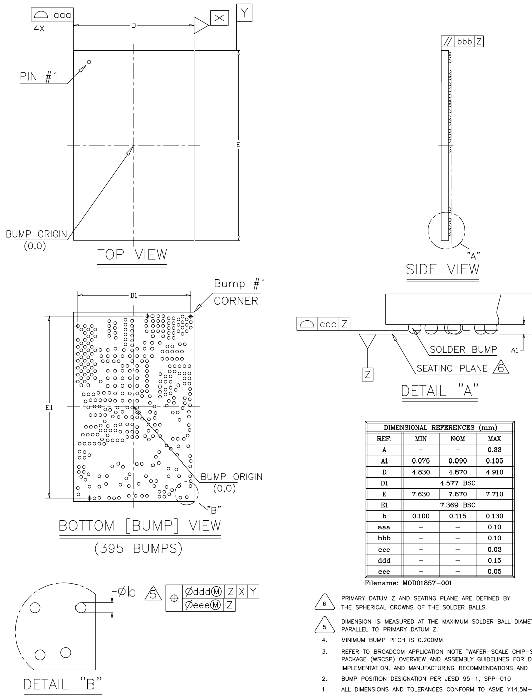
Figure 53. 395-Bump WLCSP Package
