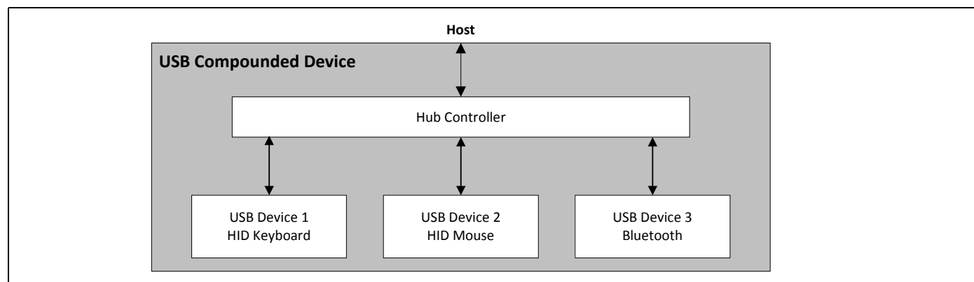
Figure 16. USB Compounded Device Configuration
