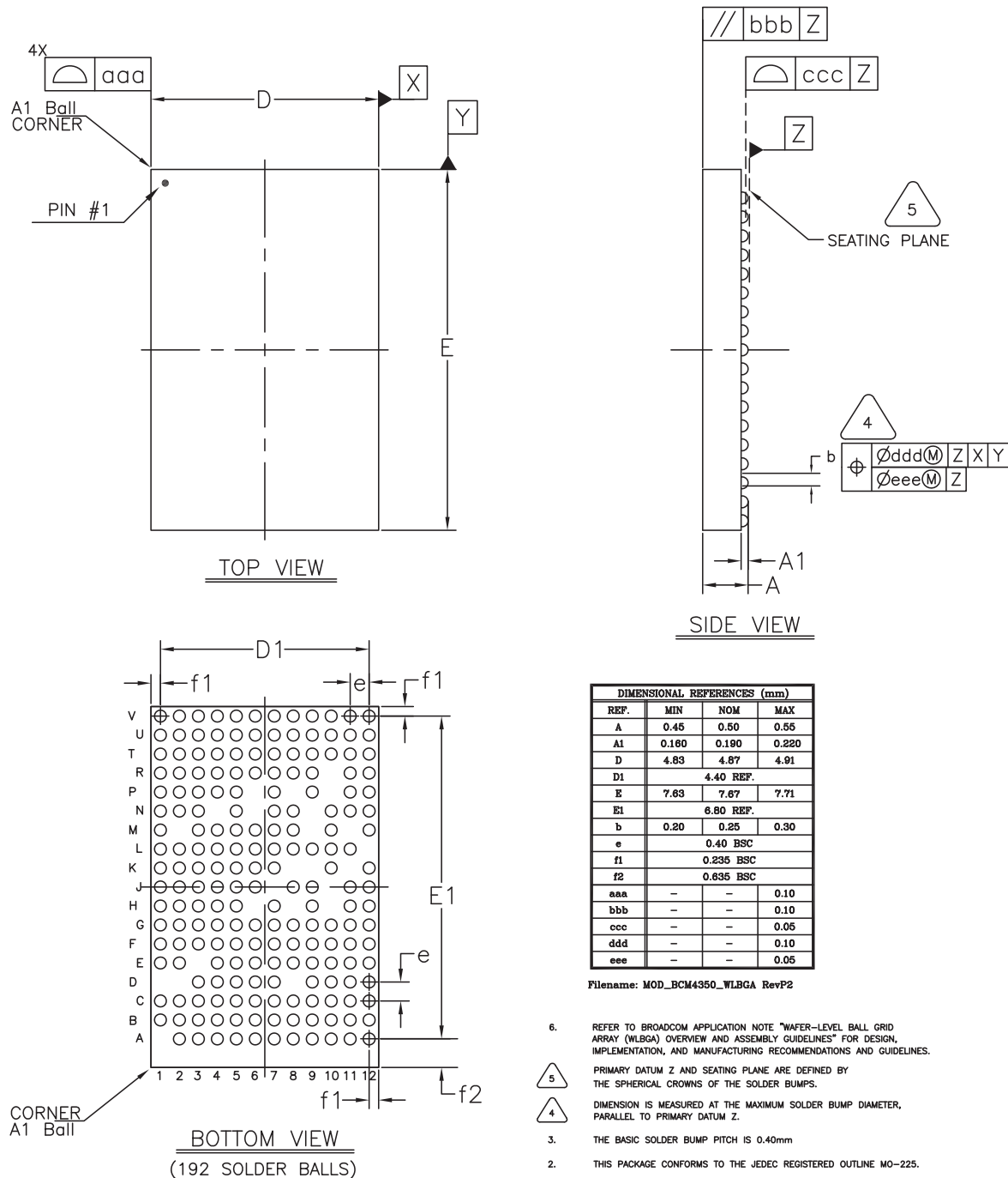
Figure 51. 192-Ball WLBGA Package Mechanical Information
