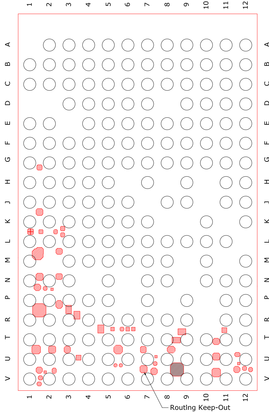
Figure 52. WLBGA Keep-Out Areas for PCB Layout (Top View, Balls Facing Down)
