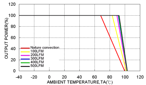
FED40-48S05 Derating Curve with Heat-sink
