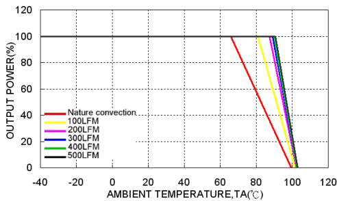
FED40-48S05 Derating Curve
