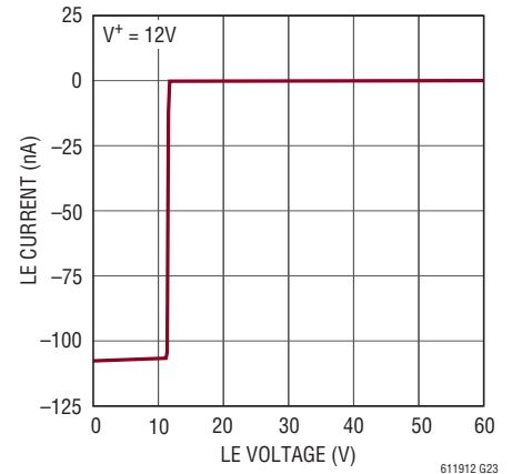
LE Current vs Voltage
