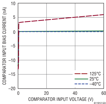
Comparator Input Bias Current vs Input Voltage
