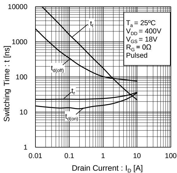
Fig.14 Switching Characteristics
