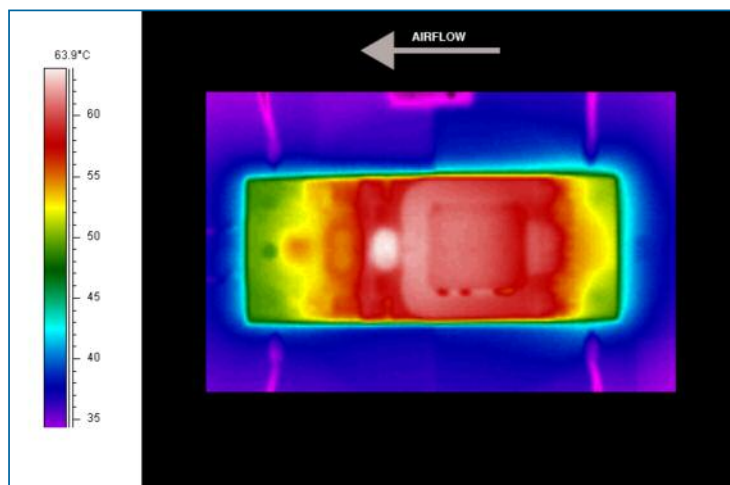
Figure 30 — Thermal plot, 600 LFM, 25 °C, 48 Vin, 450 W output power
