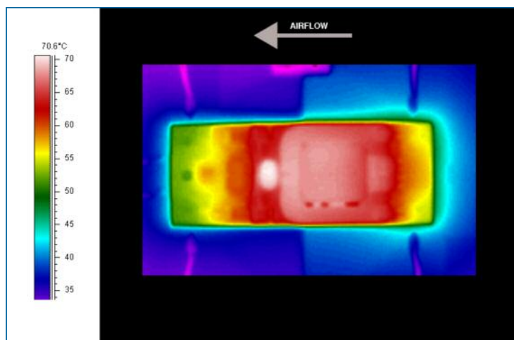
Figure 28 — Thermal plot, 400 LFM, 25 °C, 48 Vin, 450 W output power
