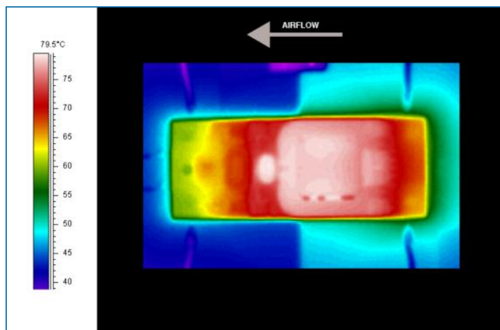
Figure 26 — Thermal plot, 200 LFM, 25 °C, 48 Vin, 450 W output power
