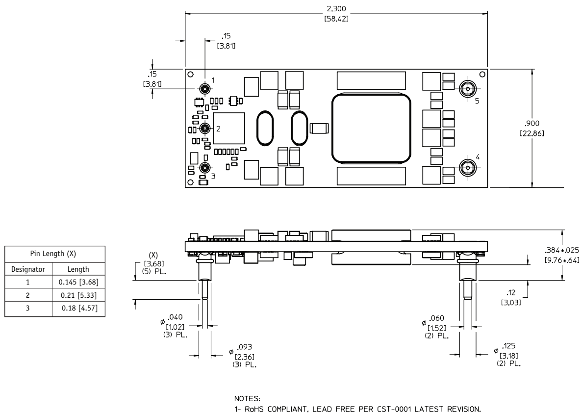
Figure 32 — IBC outline drawing
