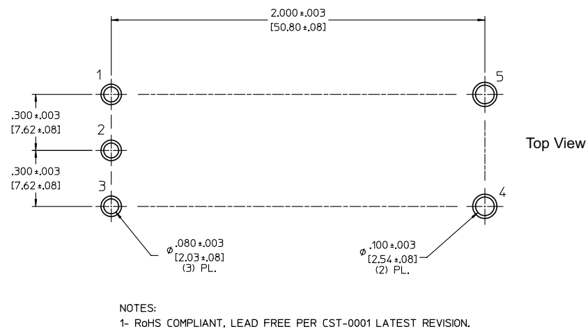
Figure 33 — IBC PCB recommended hole pattern
