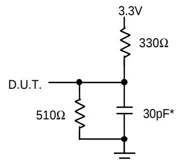
Figure 2. Output Load
