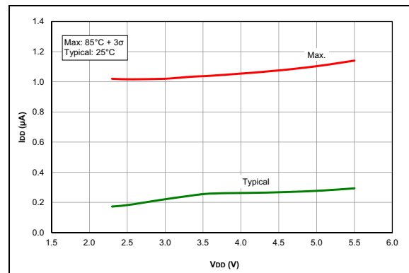
FIGURE 35-48: I_{DD} , ADC Non-Converting, PIC16F1713/6 Only.
