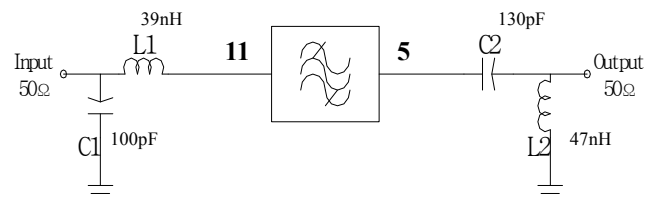
Matching Schematic
