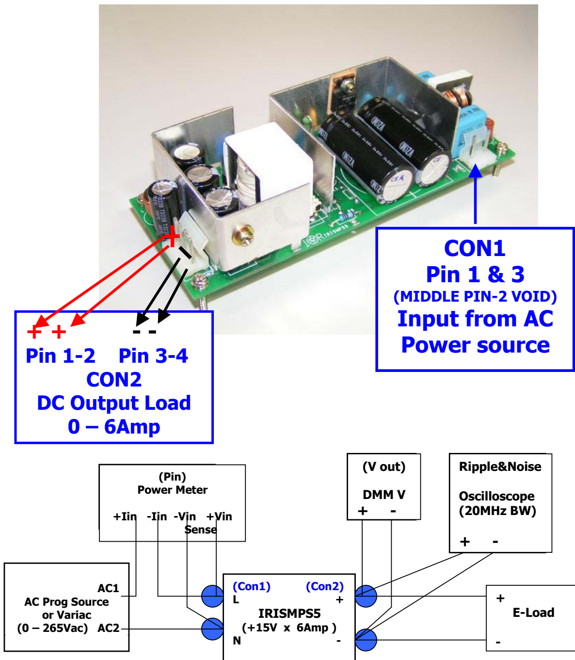
Figure 1 : Recommended test setup
