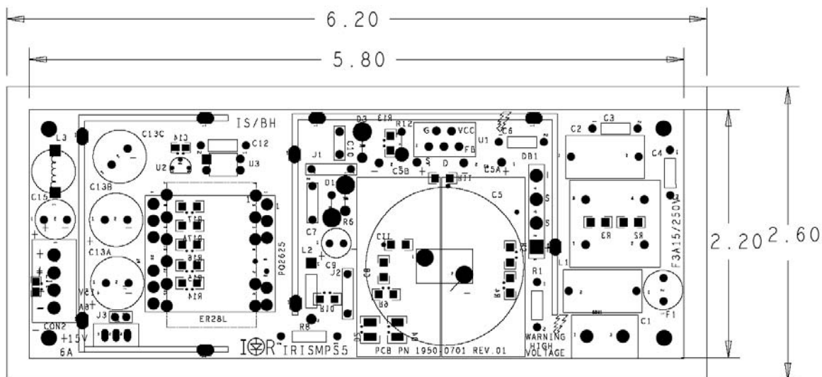
Figure 2. – Component layer of IRISMP55 demo board with physical boundary and dimensions.
