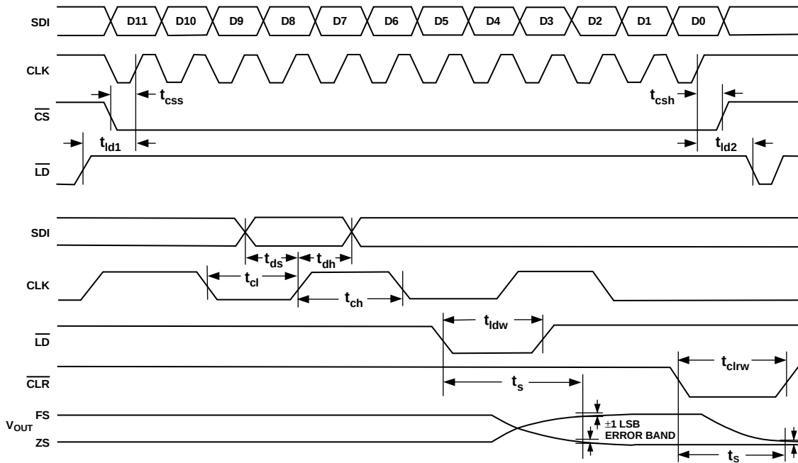
Figure 1. Timing Diagram
