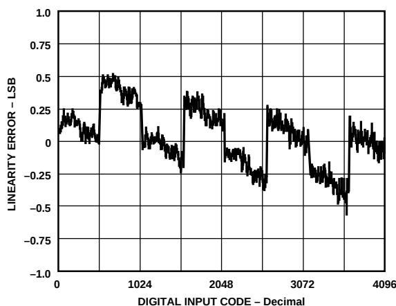
Linearity Error vs. Digital Input Code
