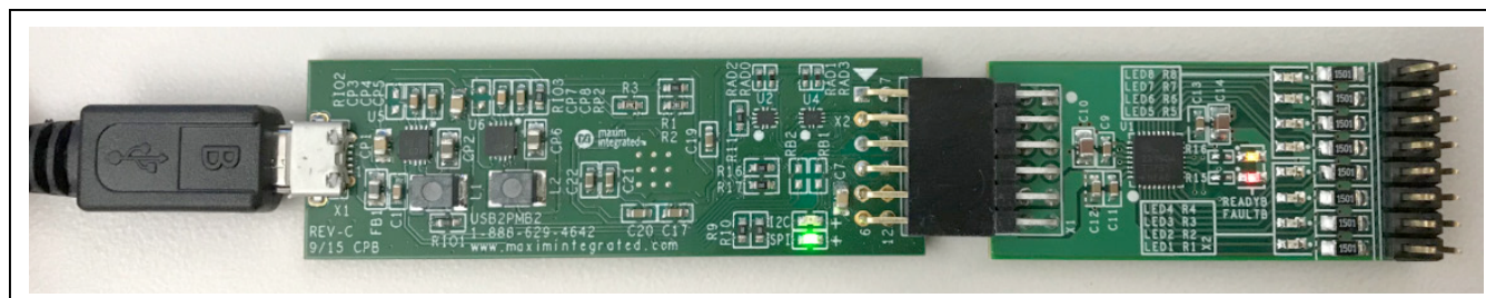
Figure 2. MAX22190PMB# with USB2PMB2# Adapter
