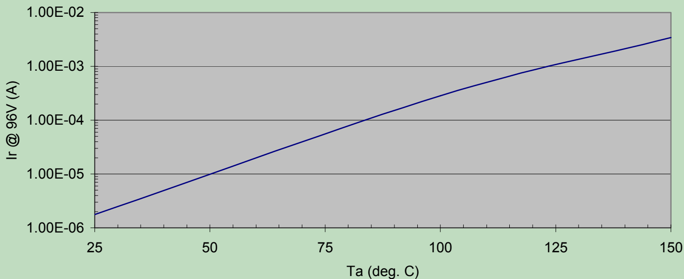
MXP1005 typical reverse current vs. temperature
