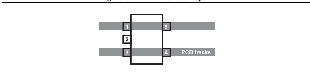
Figure 9. Recommended layout
