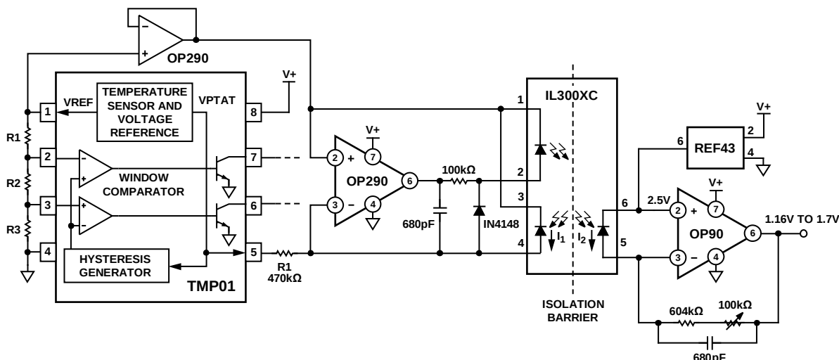
Figure 29. Isolation Amplifier
