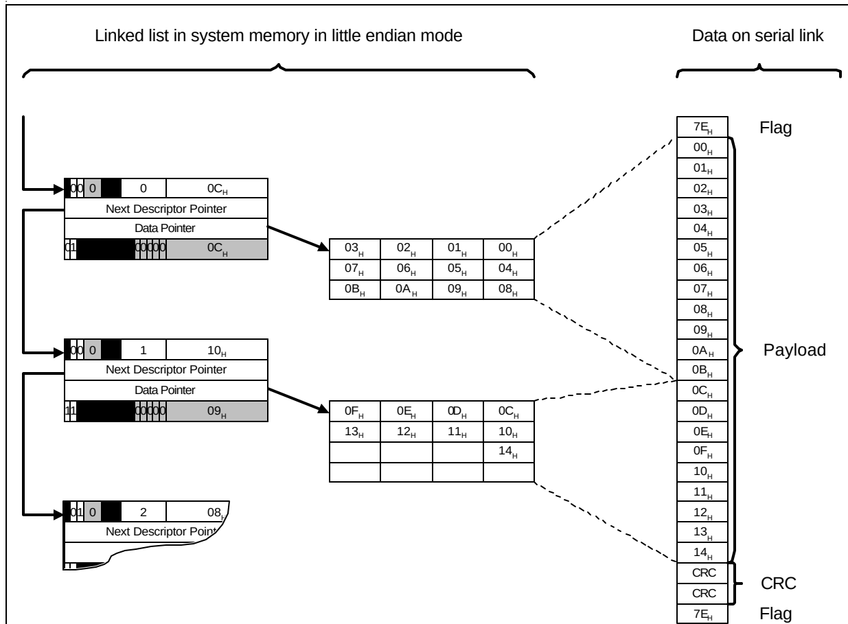
Figure 4-7 Descriptor Structure
