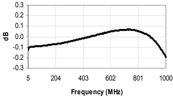
Amplitude balance
