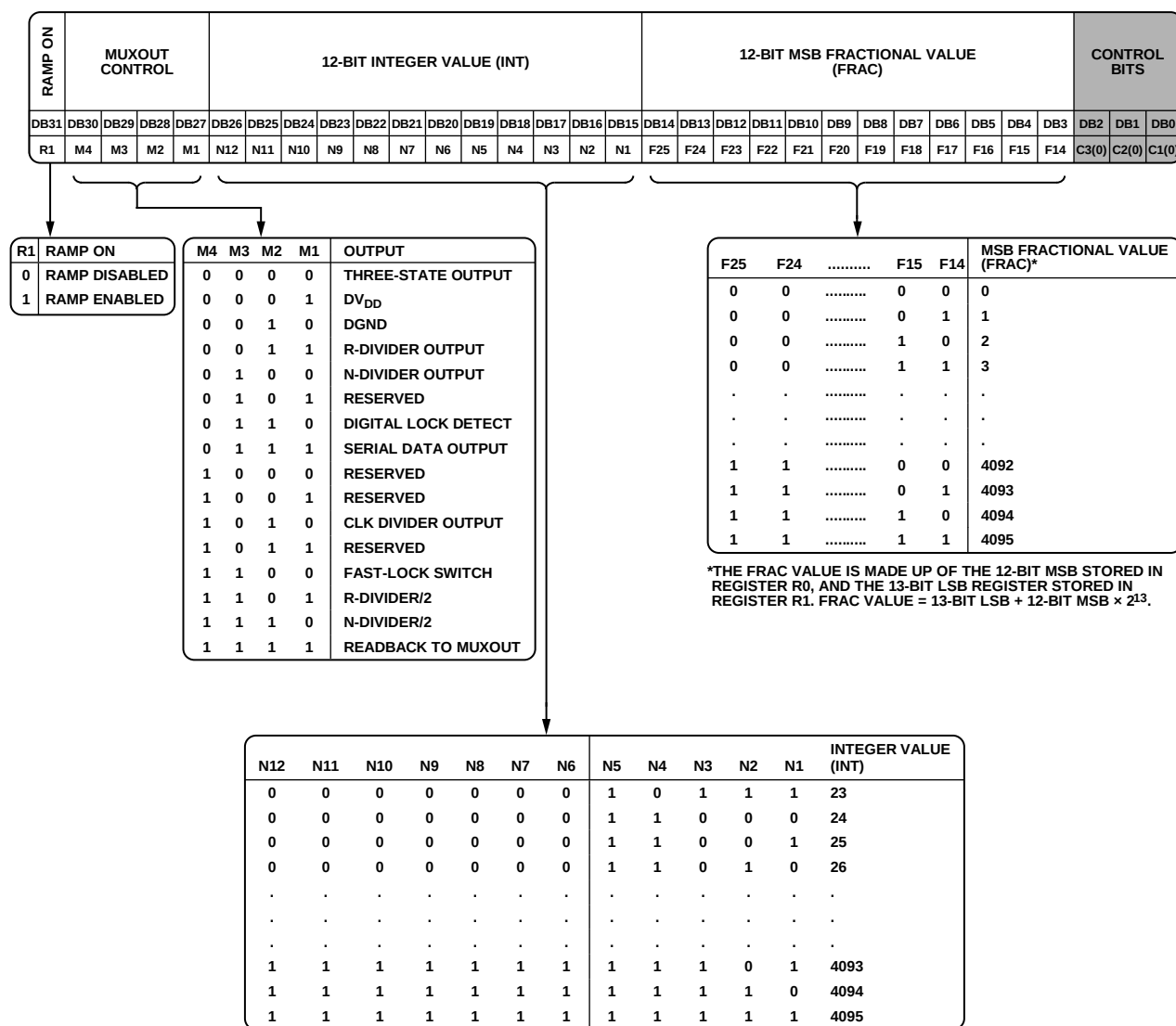
Figure 23. FRAC/INT Register (R0) Map
