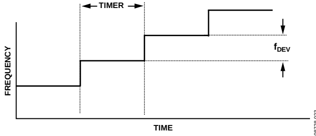
Figure 35. Waveform Timing
