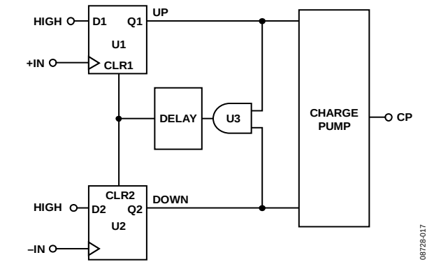
Figure 19. PFD Simplified Schematic
