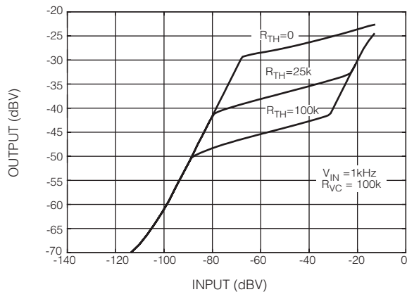
Fig. 6 Input vs Output Threshold Settings
