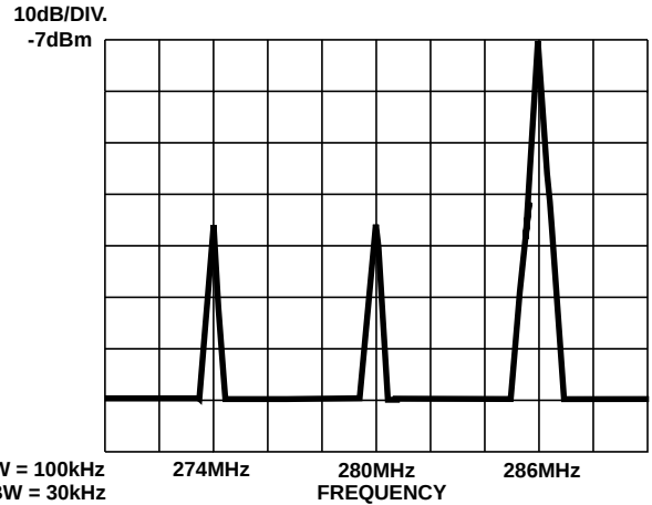
FIGURE 13. TYPICAL SSB MODULATOR RESPONSE (NOTE 3 ON AC ELECTRICAL SPECIFICATIONS, MODULATOR PERFORMANCE TABLE, LO BUFFER ENABLED)
