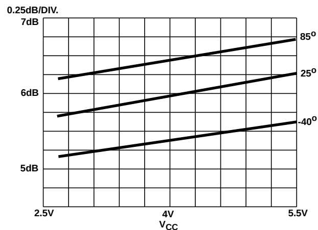
FIGURE 29. SINGLE STAGE LIMITER NOISE FIGURE vs V CC AND TEMPERATURE, R S = 250Ω, FREQUENCY = 300MHz
