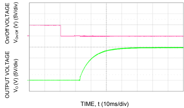
Figure 4. Typical Start-up Using Remote On/Off, negative logic version shown ( V_{IN} = 48V , I_o = I_{o,max} ).
