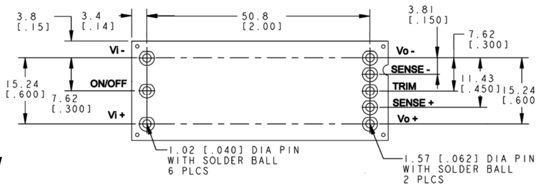
Bottom View
