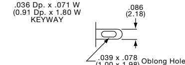
MTG406N
