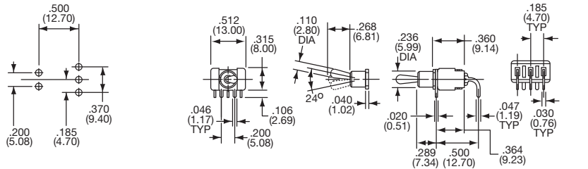
SPDT Short Toggle
