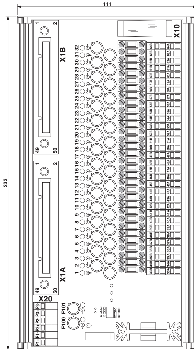
Dimensional drawing
