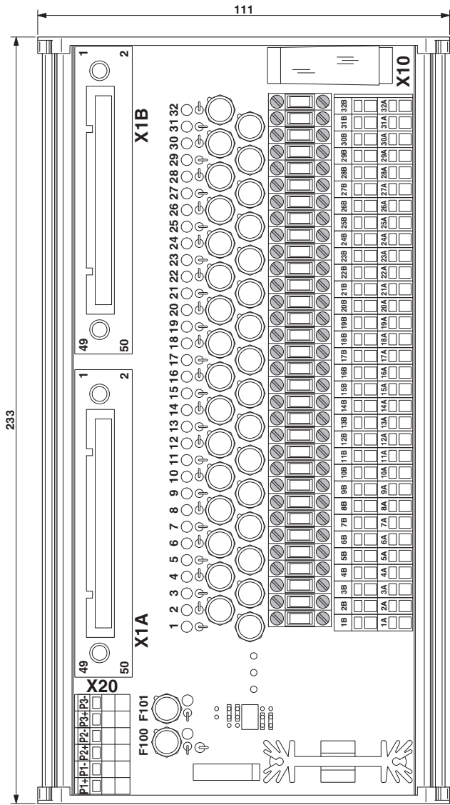
Dimensional drawing
