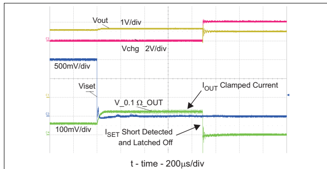
Figure 28. ISET Shorted During Normal Operation
