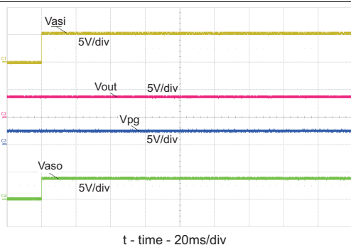
Figure 16. Power-up Timing
