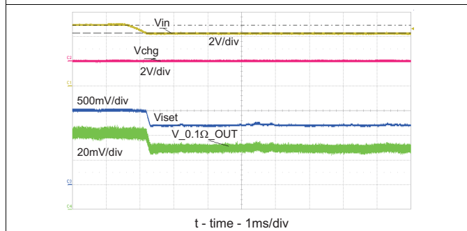
Figure 28. ISET Shorted During Normal Operation
