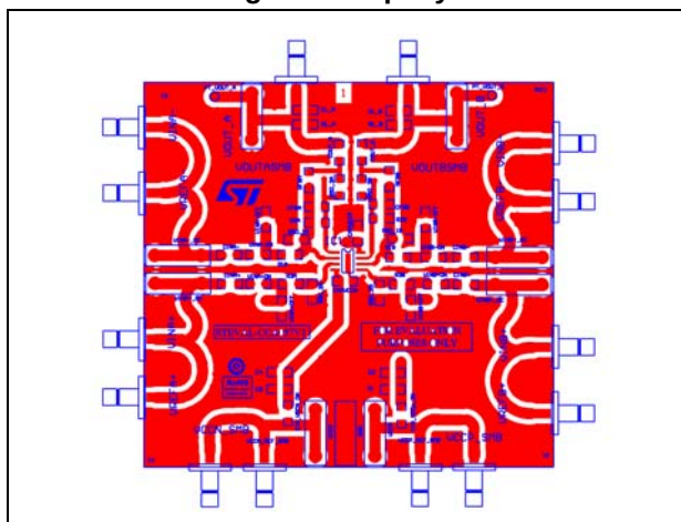
Figure 4. Top layer
