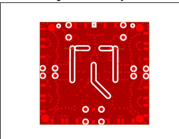
Figure 5. Bottom layer
