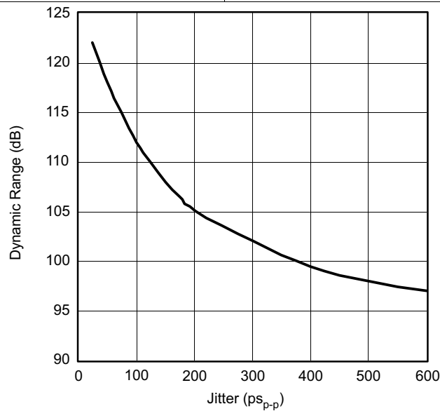
Figure 35. Jitter Dependence (x64 Oversampling)
