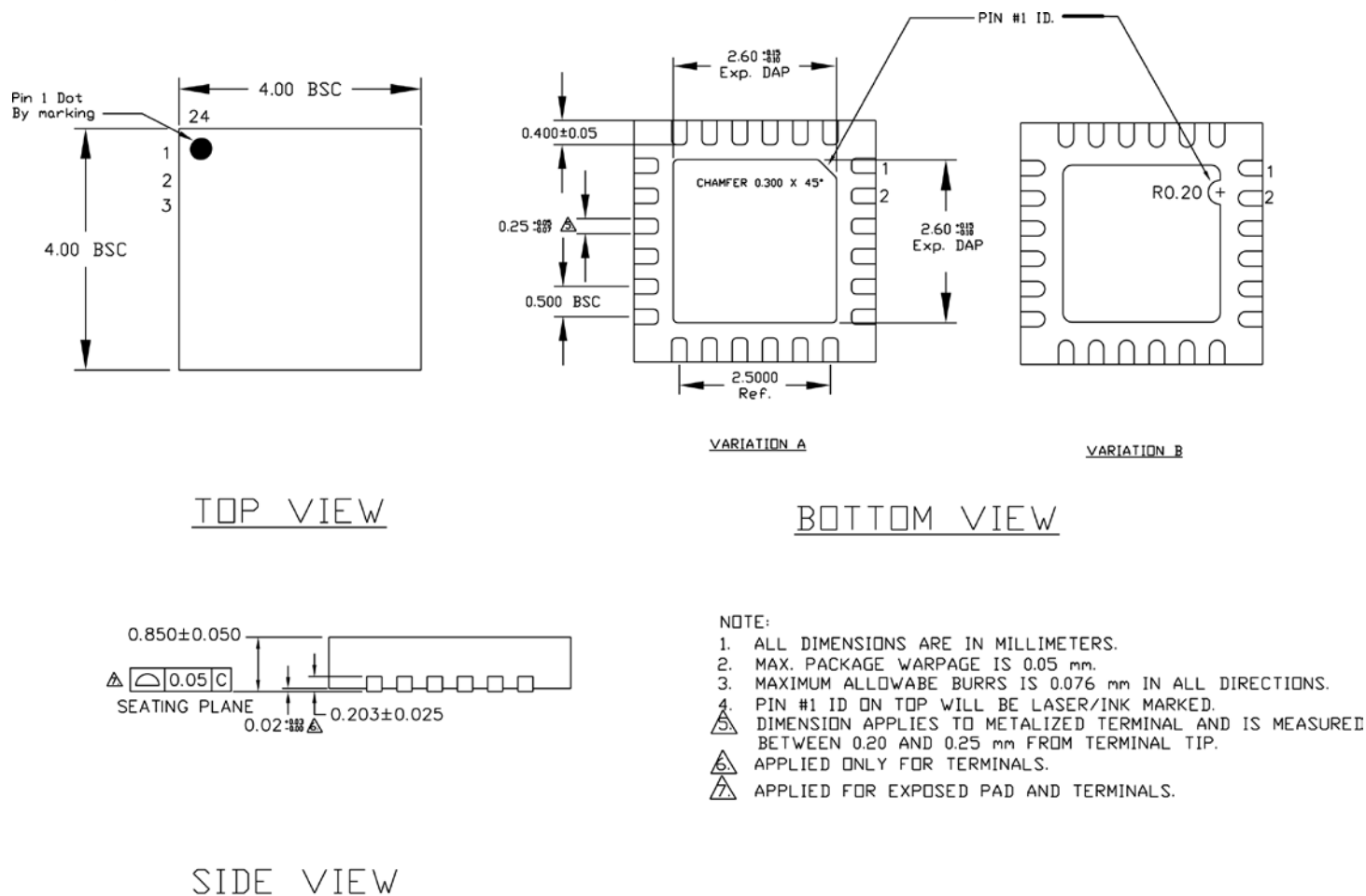
24-Pin (3mm x 3mm) QFN
