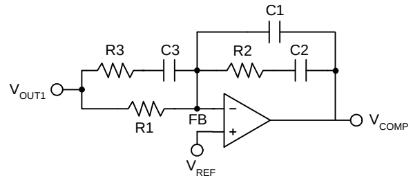
Figure 9. Compensation Network
