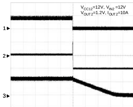
UVP_Linear Regulator ( V_{FB} < 0.4V )
