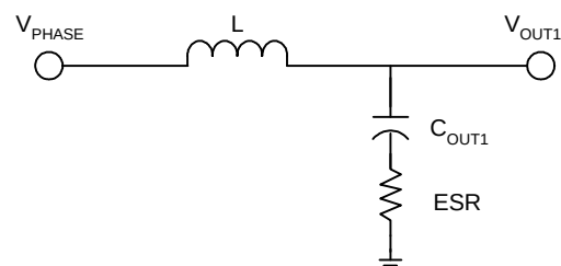
Figure 6. The Output LC Filter
