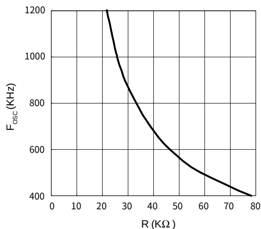
Figure 4. Oscillator Frequency vs. R_{FS\_DIS} (High Frequency)
