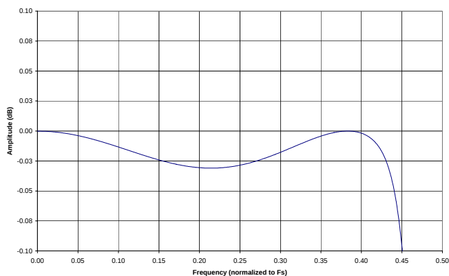
Figure 40. Double Speed Mode Passband Ripple
