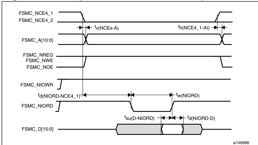
Figure 68. PC Card/CompactFlash controller waveforms for I/O space read access
