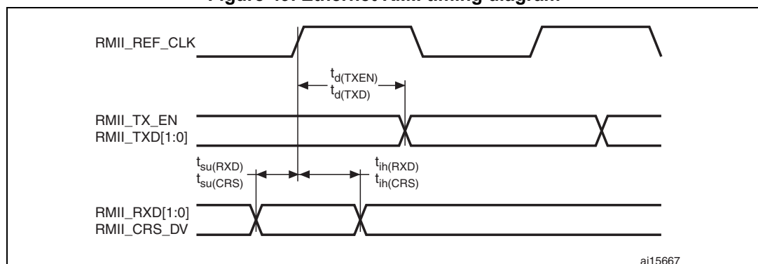
Figure 49. Ethernet RMII timing diagram
