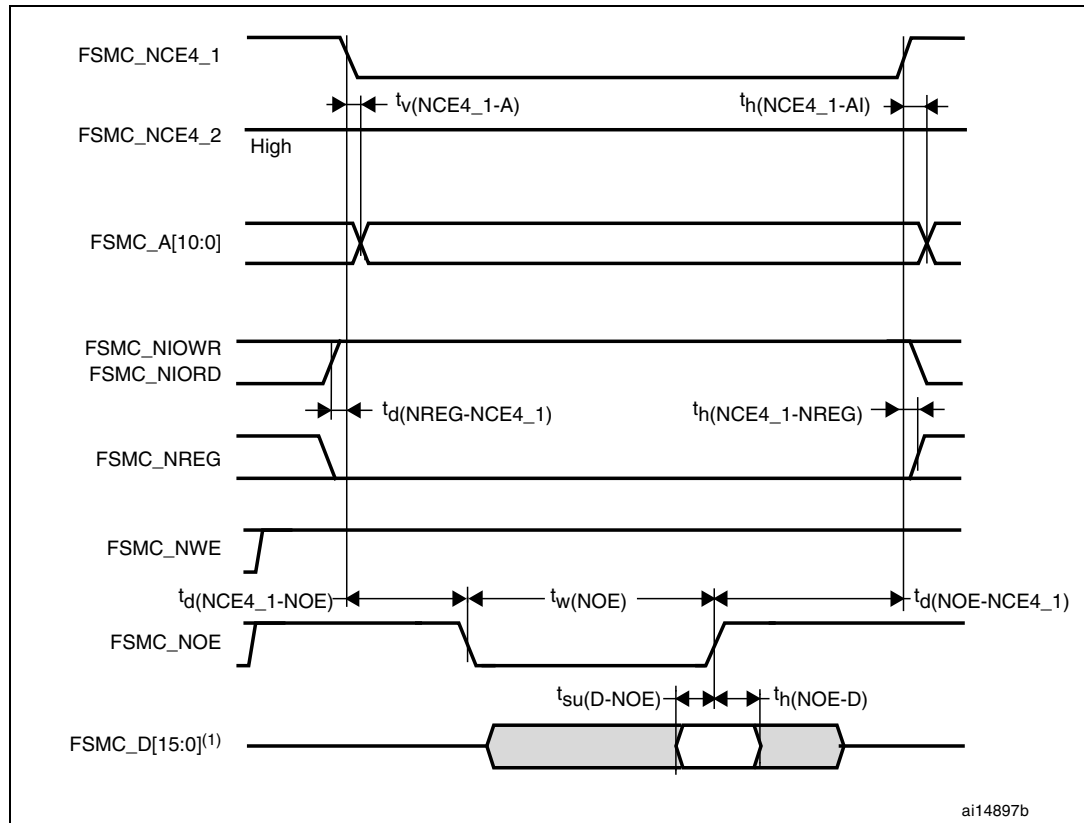
Figure 66. PC Card/CompactFlash controller waveforms for attribute memory read access
