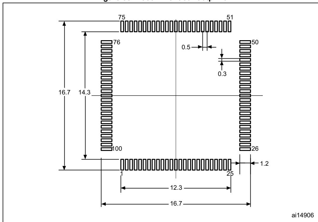
Figure 80. Recommended footprint
