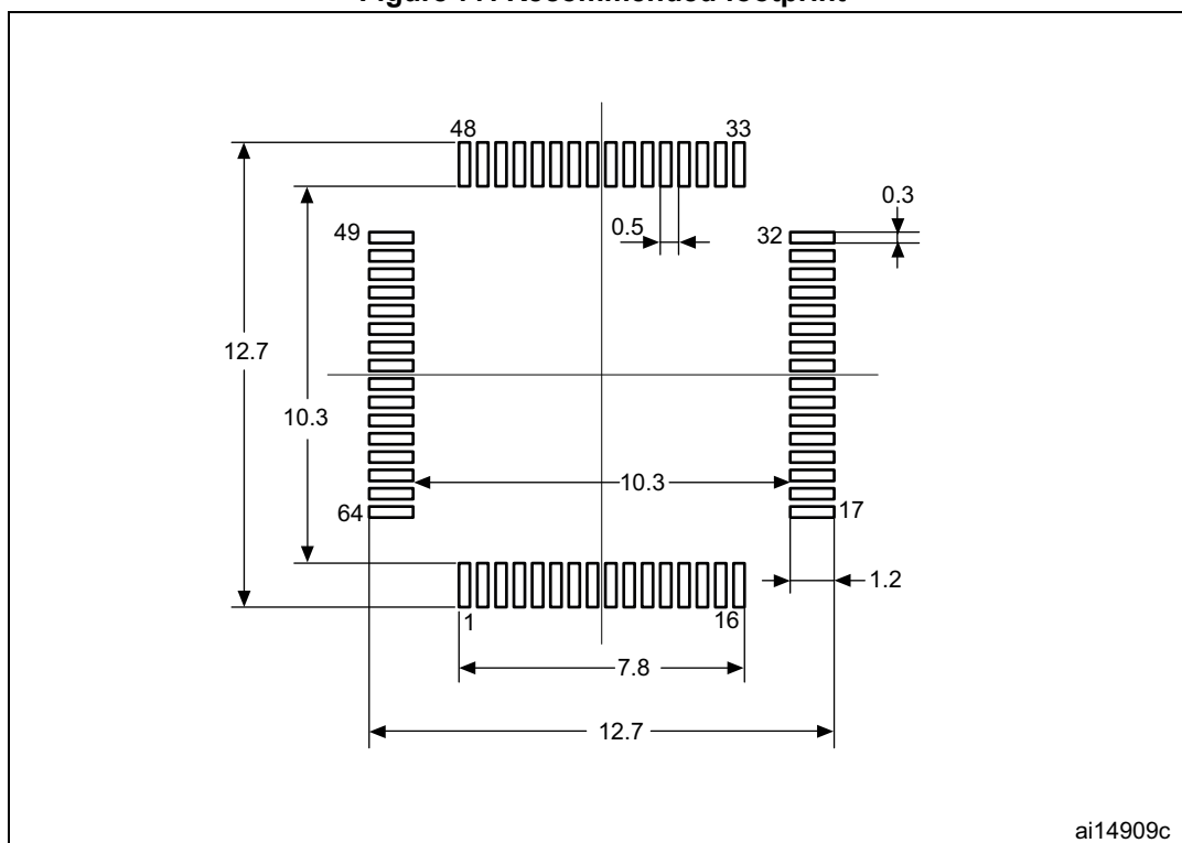
Figure 77. Recommended footprint
