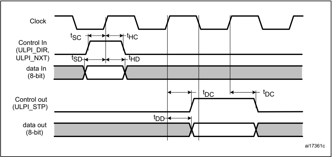
Figure 47. ULPI timing diagram
