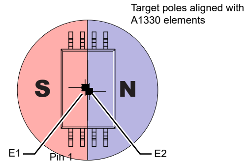
Figure 34: Orientation of Magnet Relative to Primary and Secondary Die
