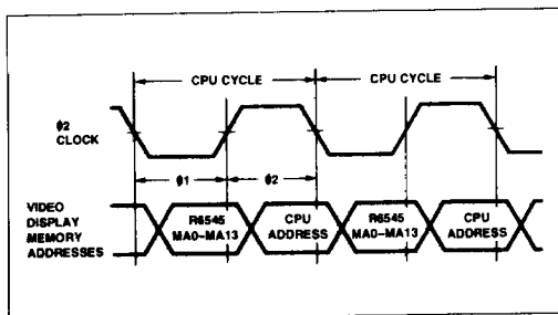
Figure 8. Ø1 and Ø2 Interleaving
