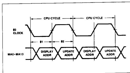
Figure 9. Ø1 and Ø2 Transparent Interleaving
