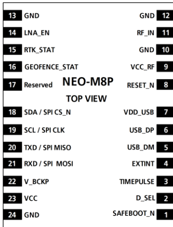
Figure 4: Pin Assignment
