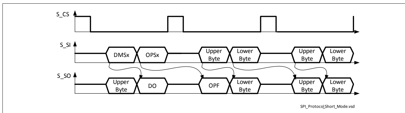
Figure 28 2x8-bit protocol
