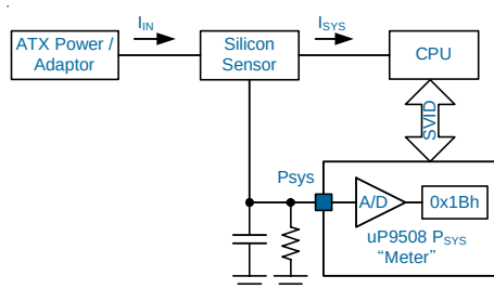
Figure 12. System Input Power Monitor
