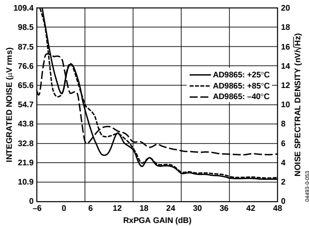
Figure 16. Input Referred Integrated Noise and Noise Spectral Density vs. RxPGA Gain (LPF f_{-3\text{dB}} = 26\text{ MHz} )
