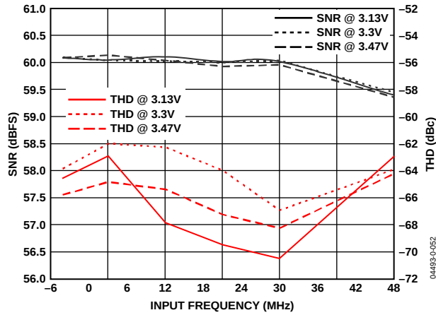
Figure 15. SNR and THD vs. Input Frequency and Supply (LPF f_{-3\text{dB}} = 26\text{ MHz} ; RxPGA = 0 dB)
