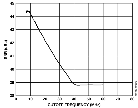
Figure 19. SNR vs. Filter Cutoff Frequency (50 MSPS; f_{\text{IN}} = 5\text{ MHz} ; \text{AIN} = -1\text{ dB} ; RxPGA = 48 dB)
