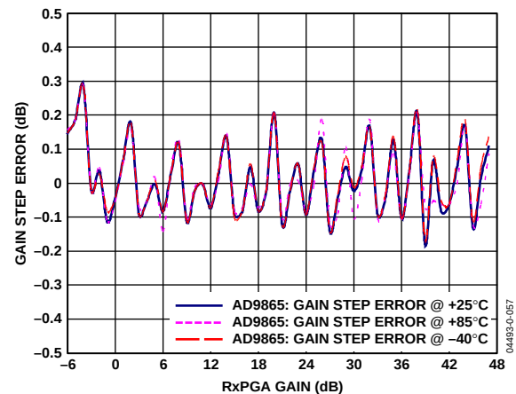
Figure 20. RxPGA Gain Step Error vs. Gain ( f_{\text{IN}} = 10\text{ MHz} )
