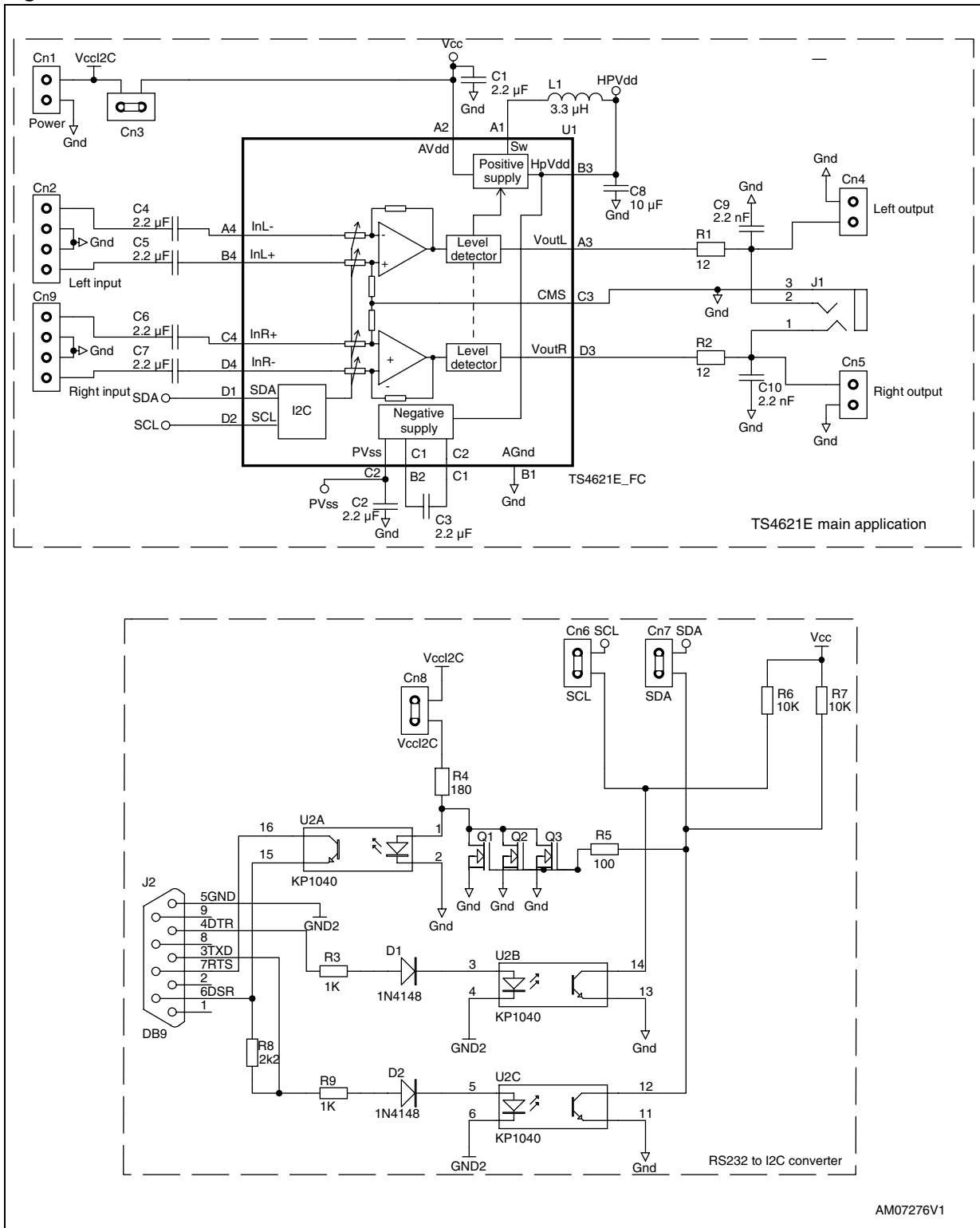
Figure 1. Circuit schematics
