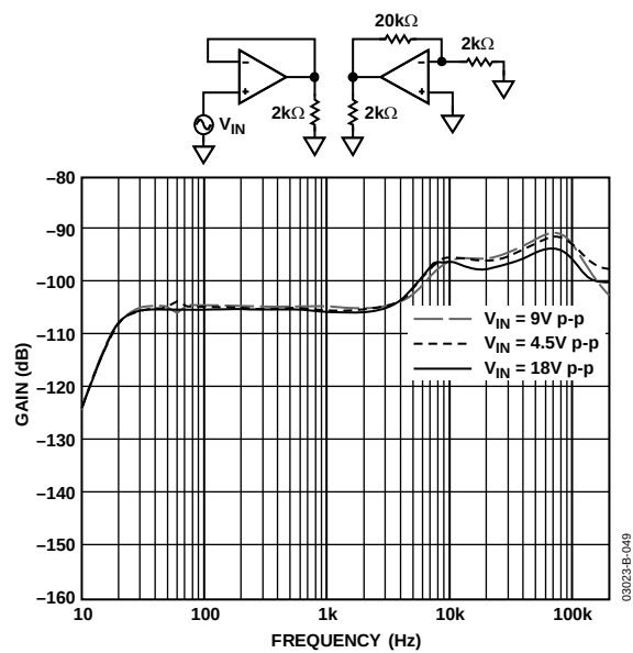
Figure 38. Channel Separation
