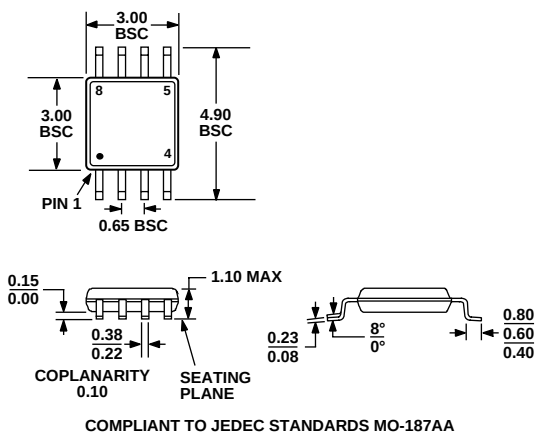
Figure 52. 8-Lead Mini Small Outline Package [MSOP] (RM-8)
