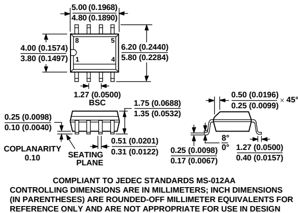
Figure 51. 8-Lead Standard Small Outline Package [SOIC] Narrow Body (R-8)
