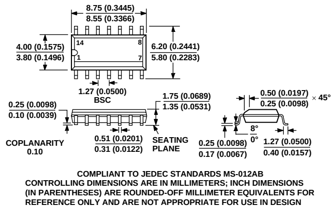
Figure 53. 14-Lead Standard Small Outline Package [SOIC] Narrow Body (R-14)
