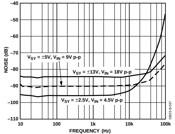
Figure 37. Total Harmonic Distortion + Noise vs. Frequency
