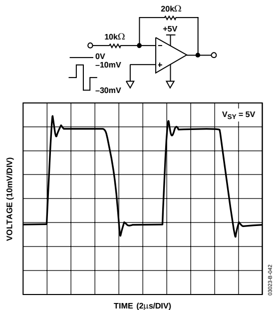
Figure 43. Gain of Two Inverter Response to 20 mV Step, Centered 20 mV below Ground
