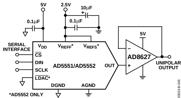
Figure 46. Unipolar Output
