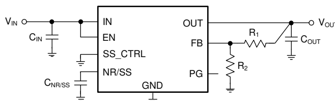
Figure 38. Adjustable Operation
