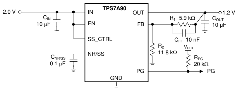
Figure 39. Application Example
