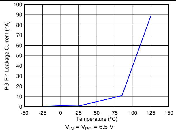
Figure 24. PG Leakage Current vs Temperature
