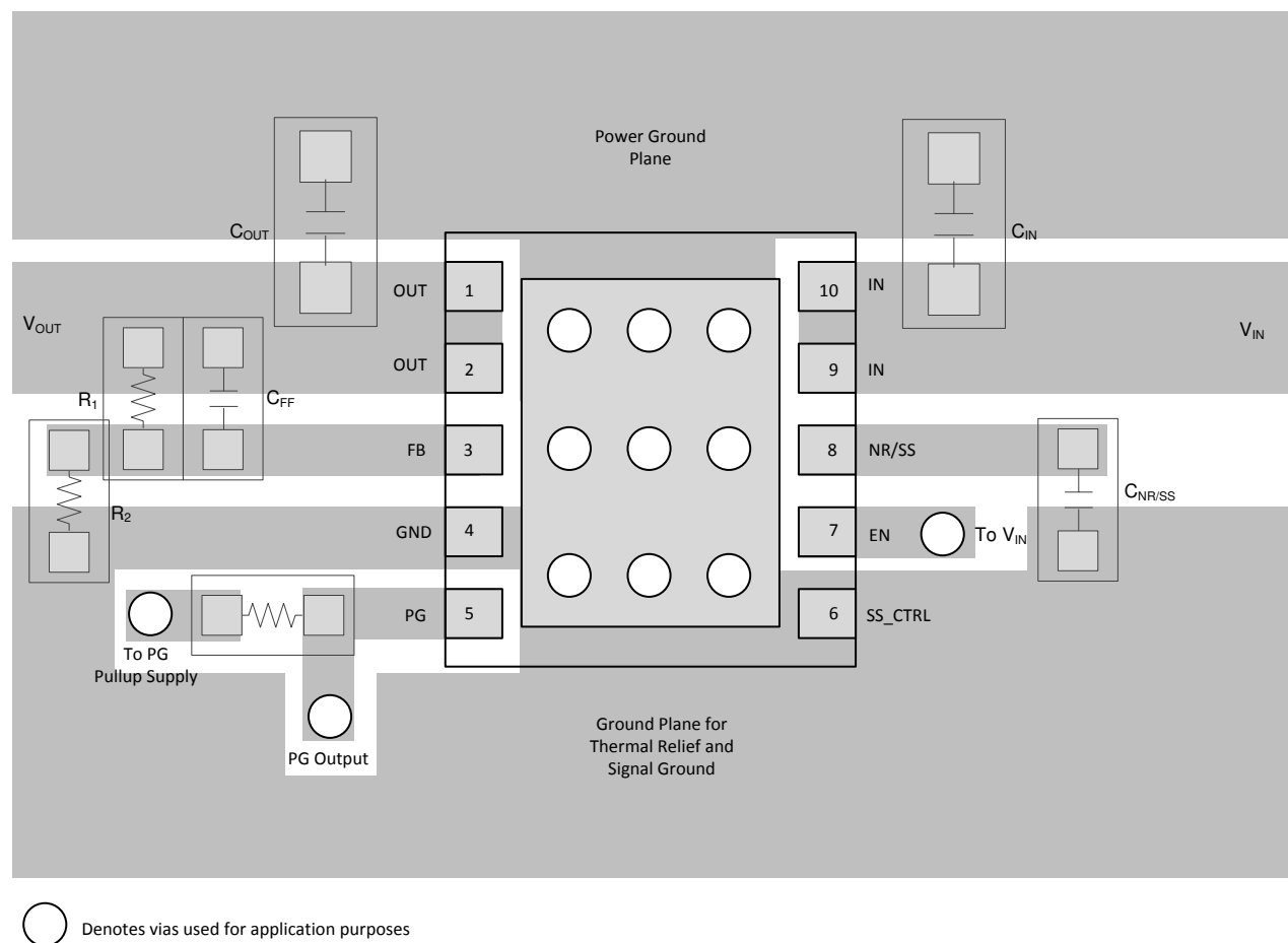
Figure 42. TPS7A90 Example Layout
