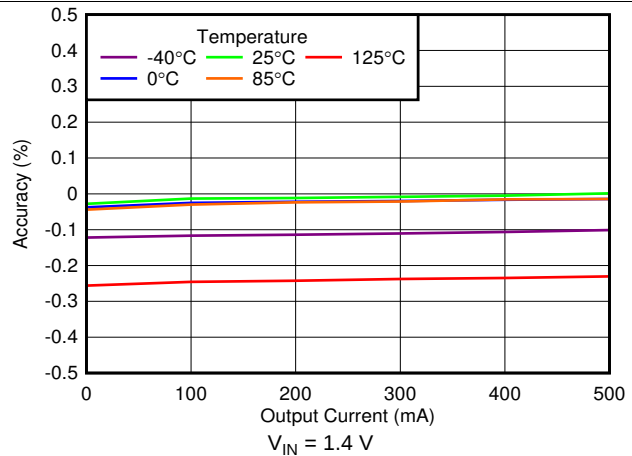
Figure 16. Load Regulation
