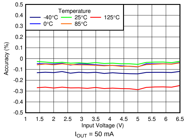
Figure 17. Line Regulation
