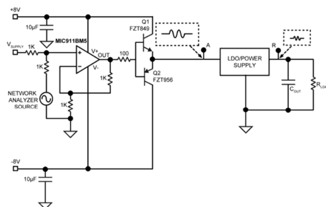
Figure 3. Network Analyzer Set-Up
